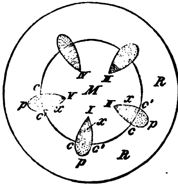
Fig. 3.—Diagram showing the position of the woody bundles, I, II , etc.
